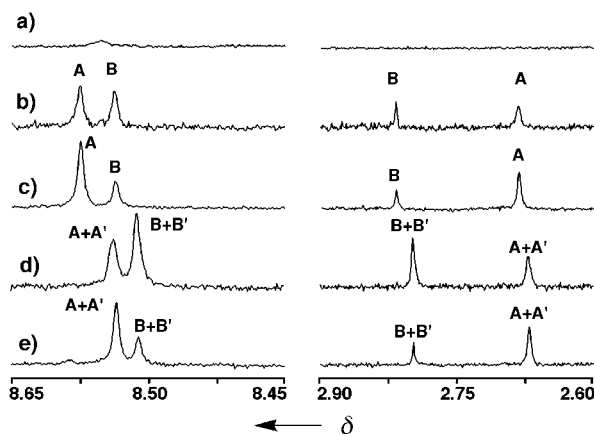
Figure 1. Portions of the ^1\text{H} NMR spectra showing the selected NH peaks of the dimer (8.65–8.45 ppm) and \text{H}_a peaks for the guest inside the capsules (2.90–2.60 ppm). The labels A and A' denote the thermodynamically more-stable complexes of (+)- 2 and (–)- 2 , respectively, while B and B' denote the respective less-stable complexes. a) 1b·1b in [\text{D}_{10}]p -xylene ( 8.25 \times 10^{-4} \text{ M} ); b) 4 min and c) 120 h after addition of 3 equiv of (+)- 2 ; d) 17 min and e) 191 h after addition of 30 equiv of (–)- 2 .
